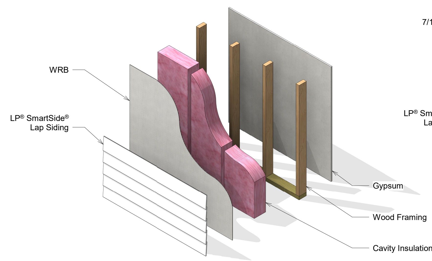
① Exploded Isometric 1 - Direct to Stud Application
