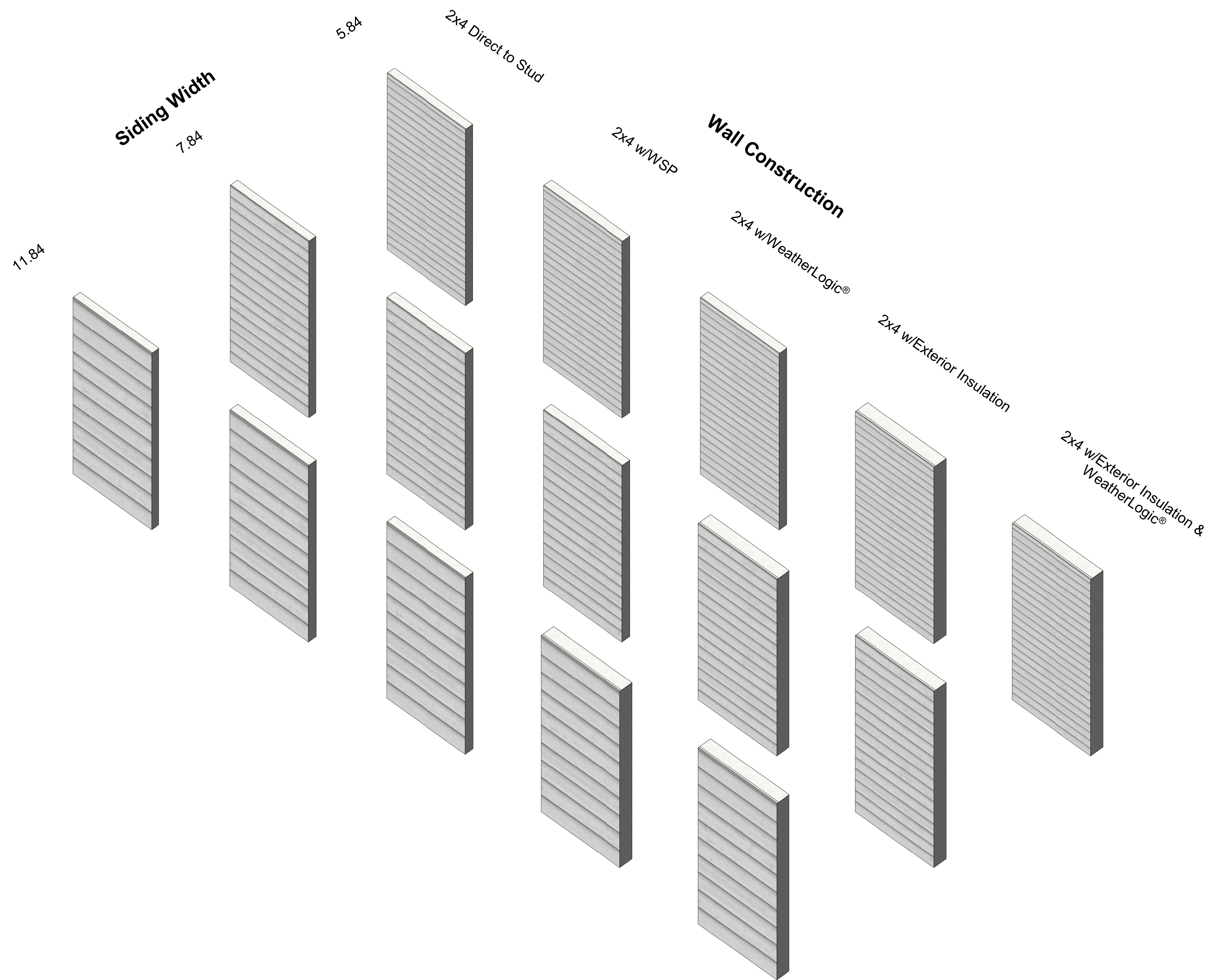
① Wall Types 2 - 76 Series Cedar Texture Lap (Strand)
