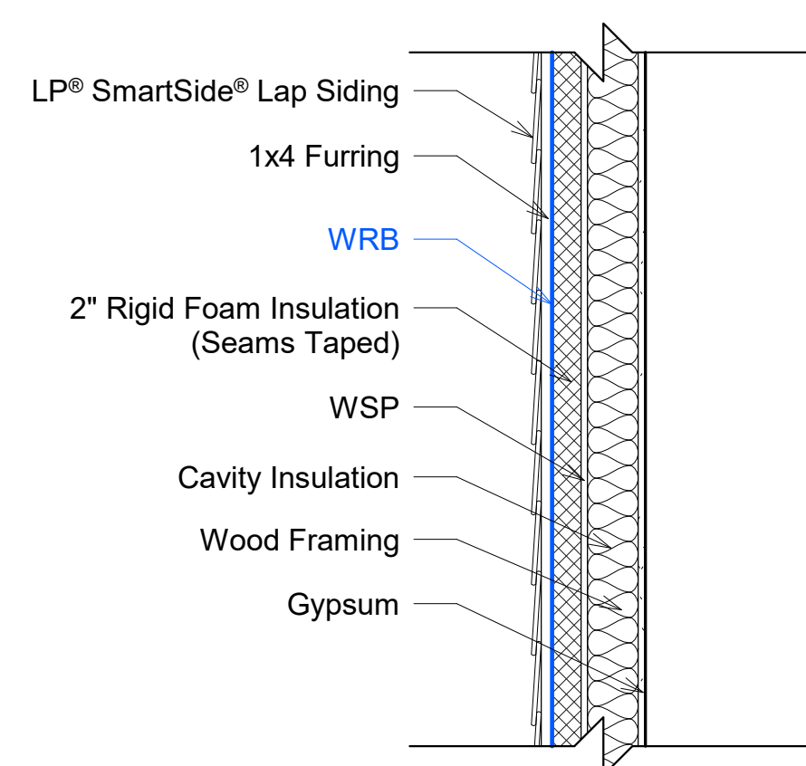
3 Section 4 - Exterior Insulation Application 1 1" = 1'-0"
