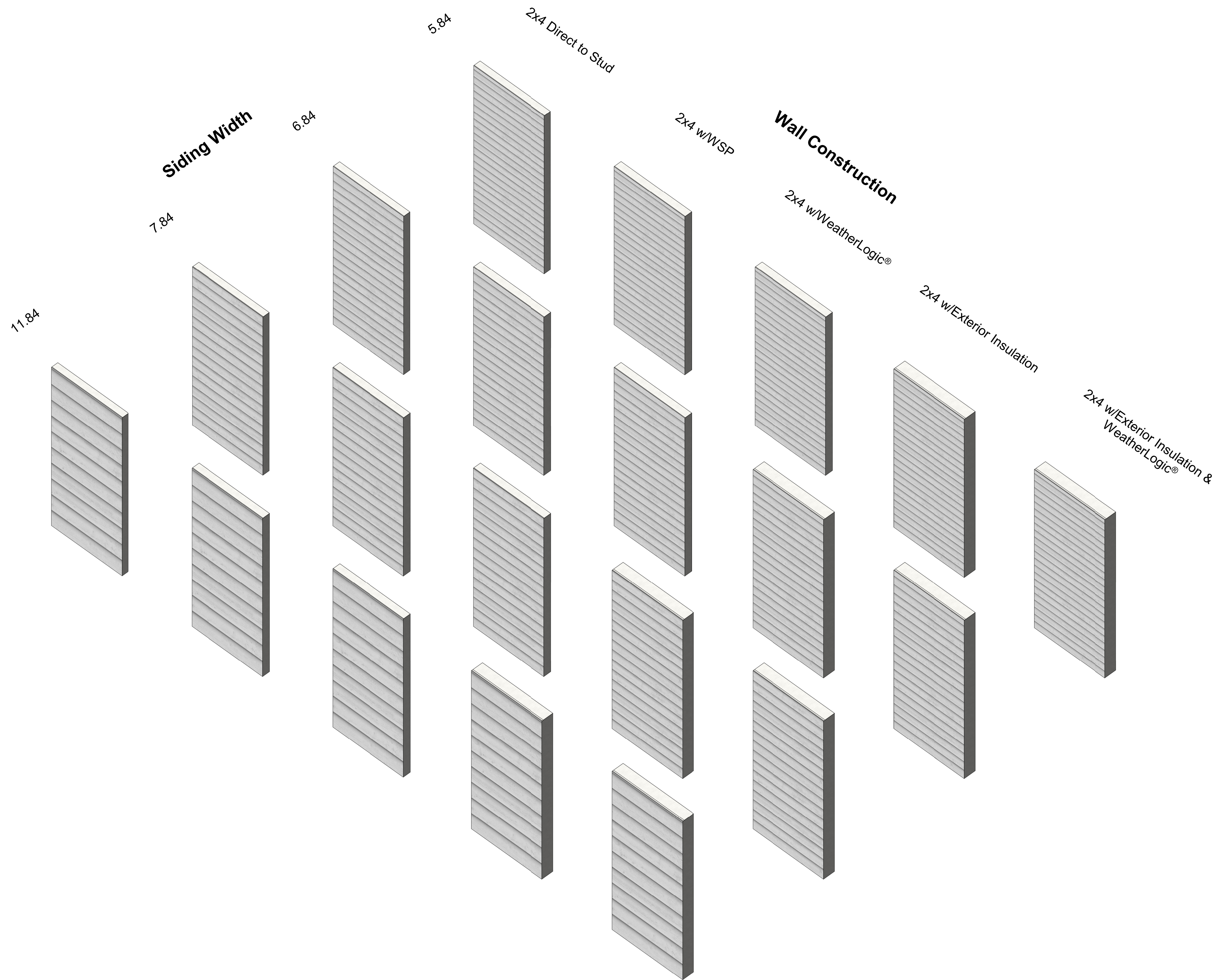
1 Wall Types 1 - 38 Series Cedar Texture Lap (Strand)
