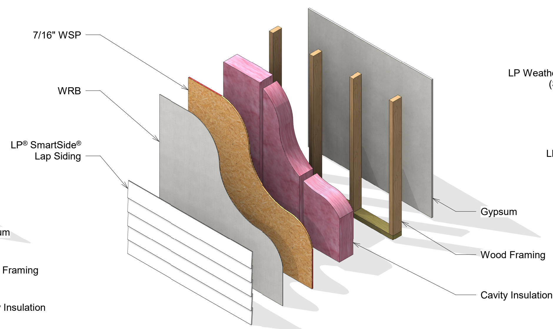
② Exploded Isometric 2 - WSP Application
