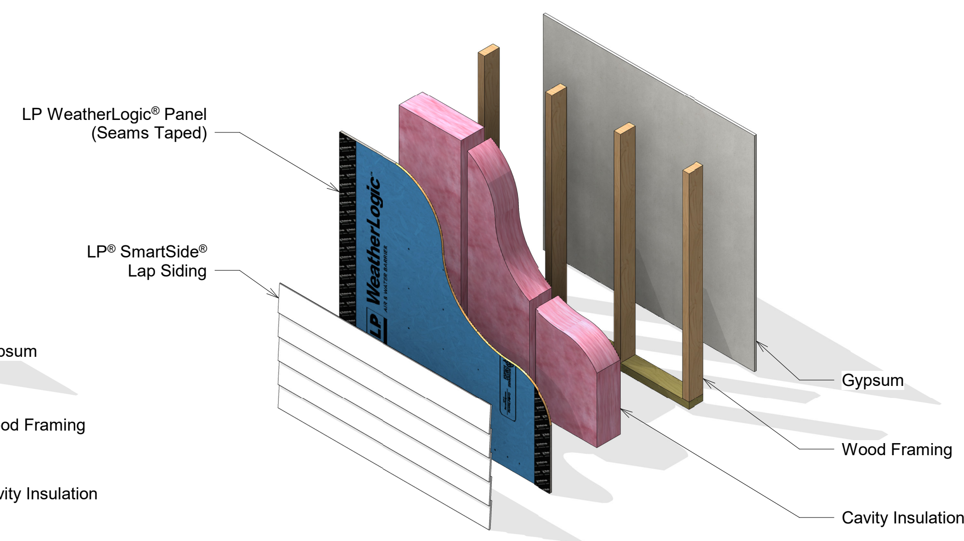
③ Exploded Isometric 3 - WeatherLogic® Application
