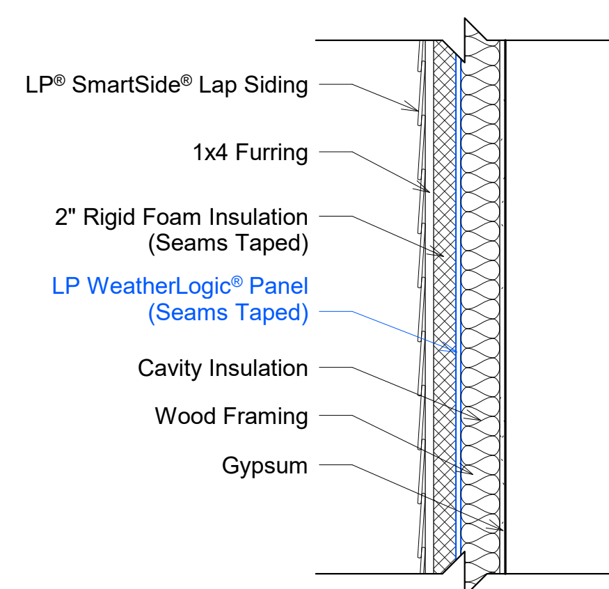
4 Section 5 - Exterior Insulation Application 2 1" = 1'-0"
