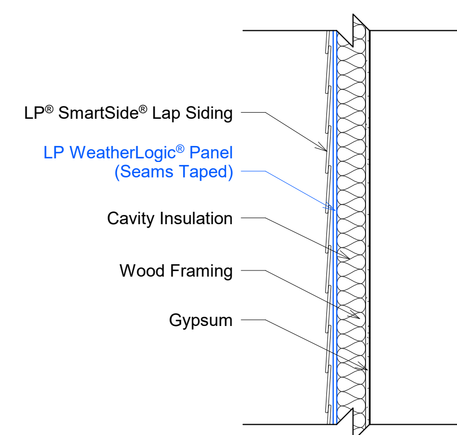
⑥ Section 3 - WeatherLogic® Application 1" = 1'-0"
