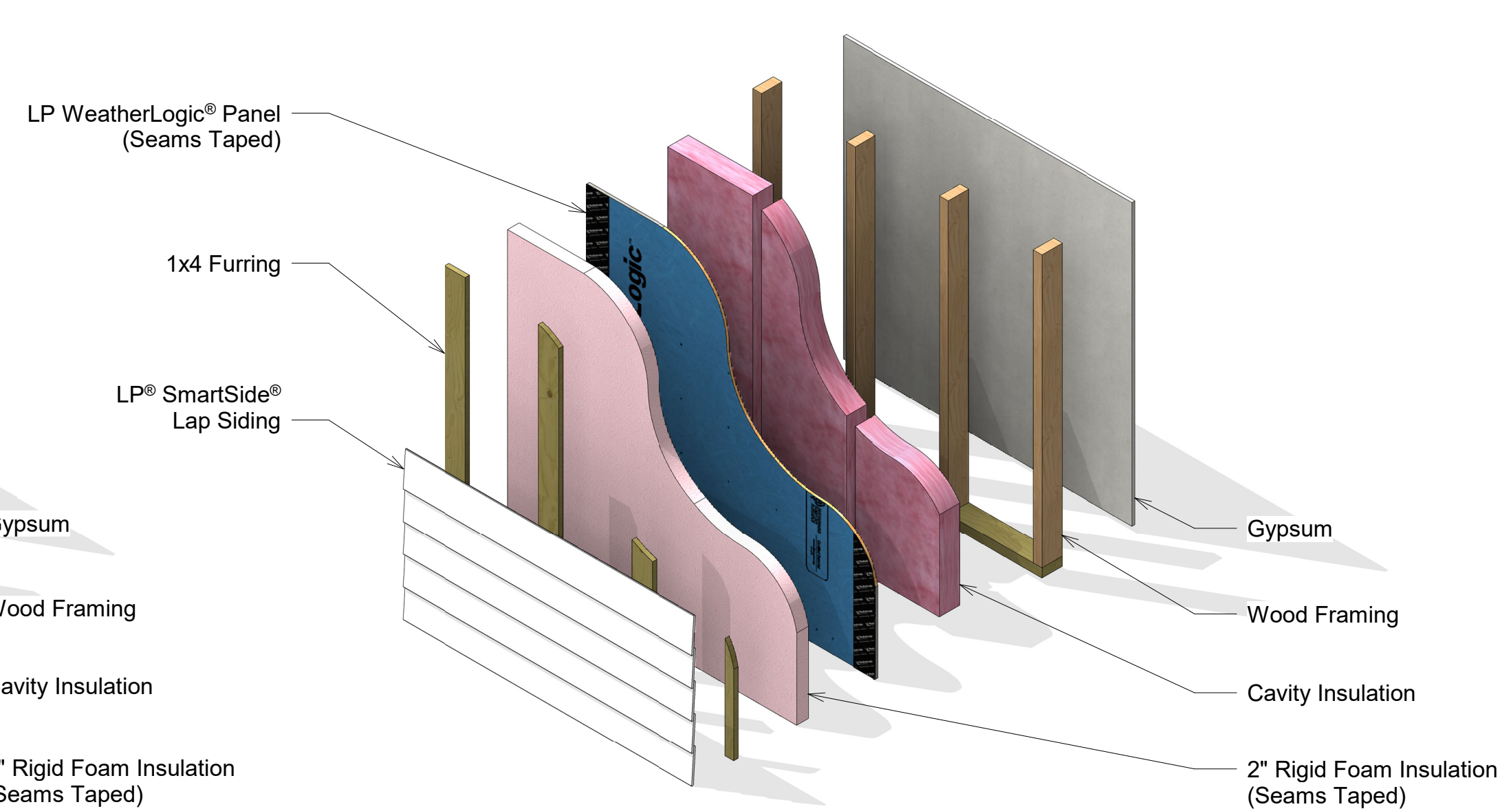
2 Exploded Isometric 5 - Exterior Insulation Application 2
