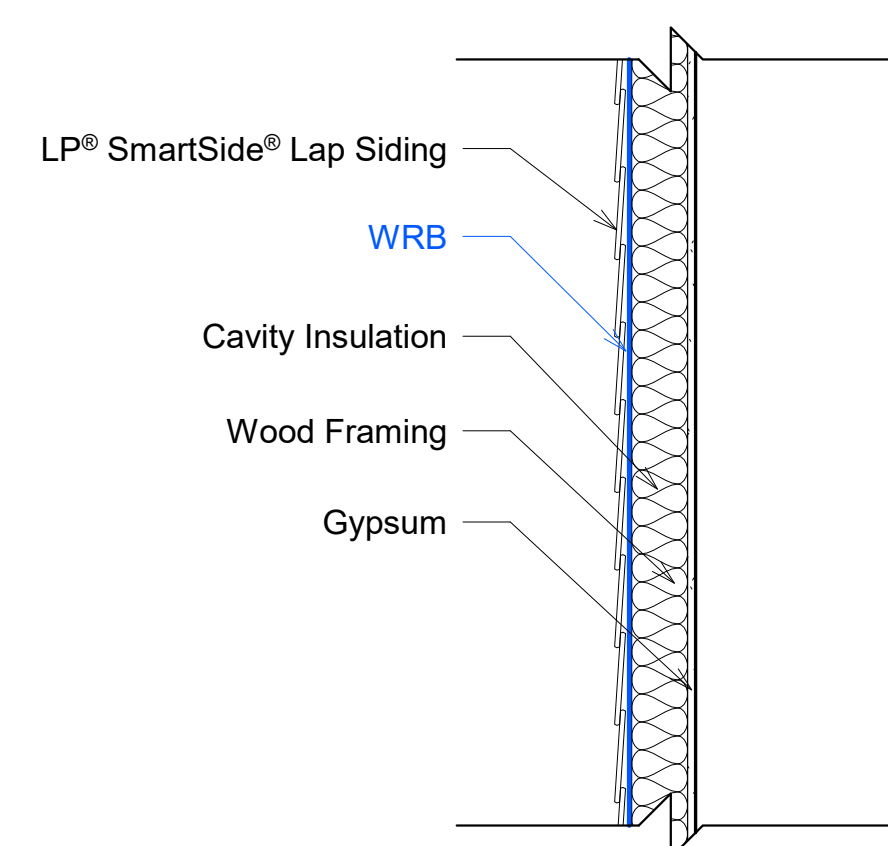
④ Section 1 - Direct to Stud Application 1" = 1'-0"
