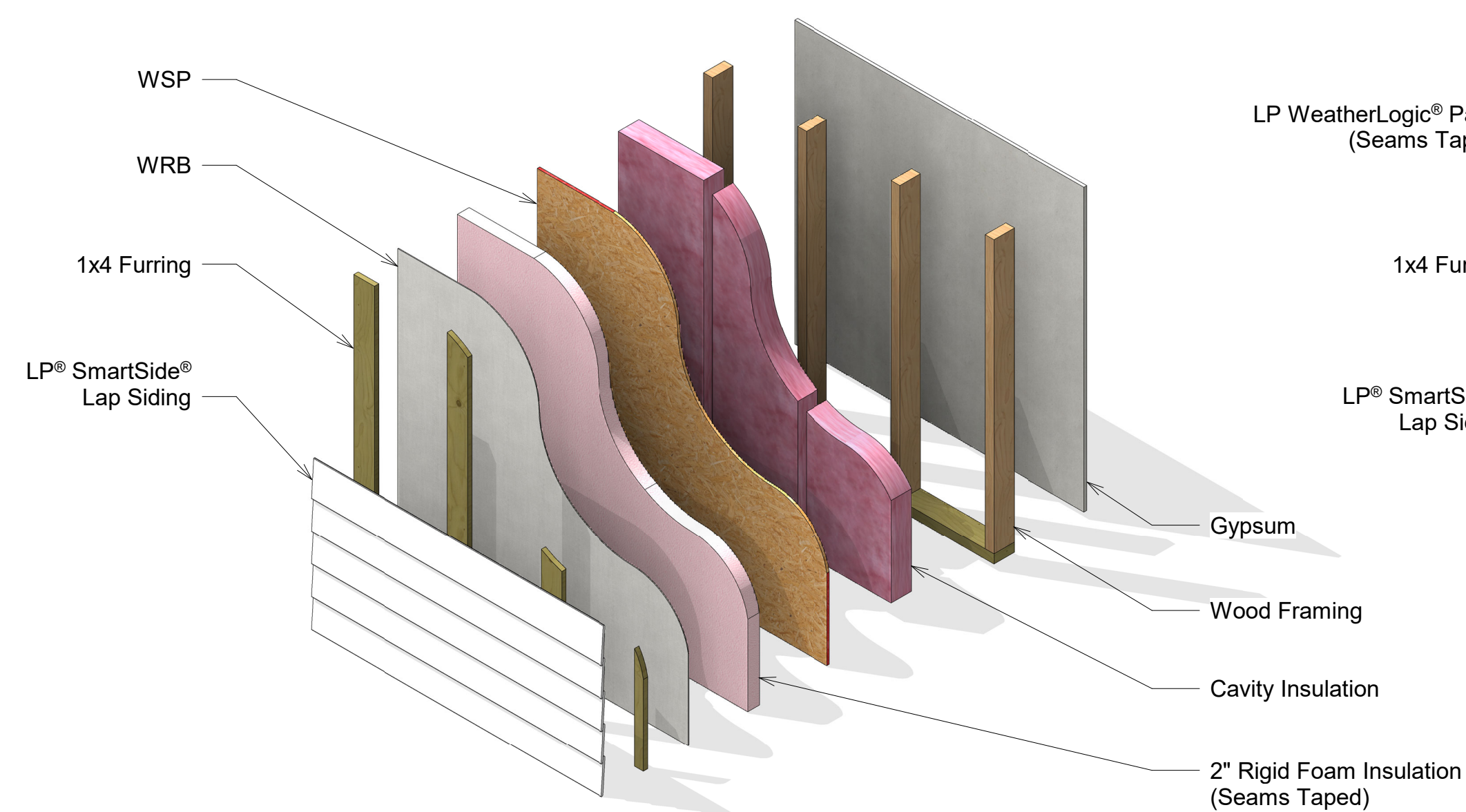
1 Exploded Isometric 4 - Exterior Insulation Application 1
