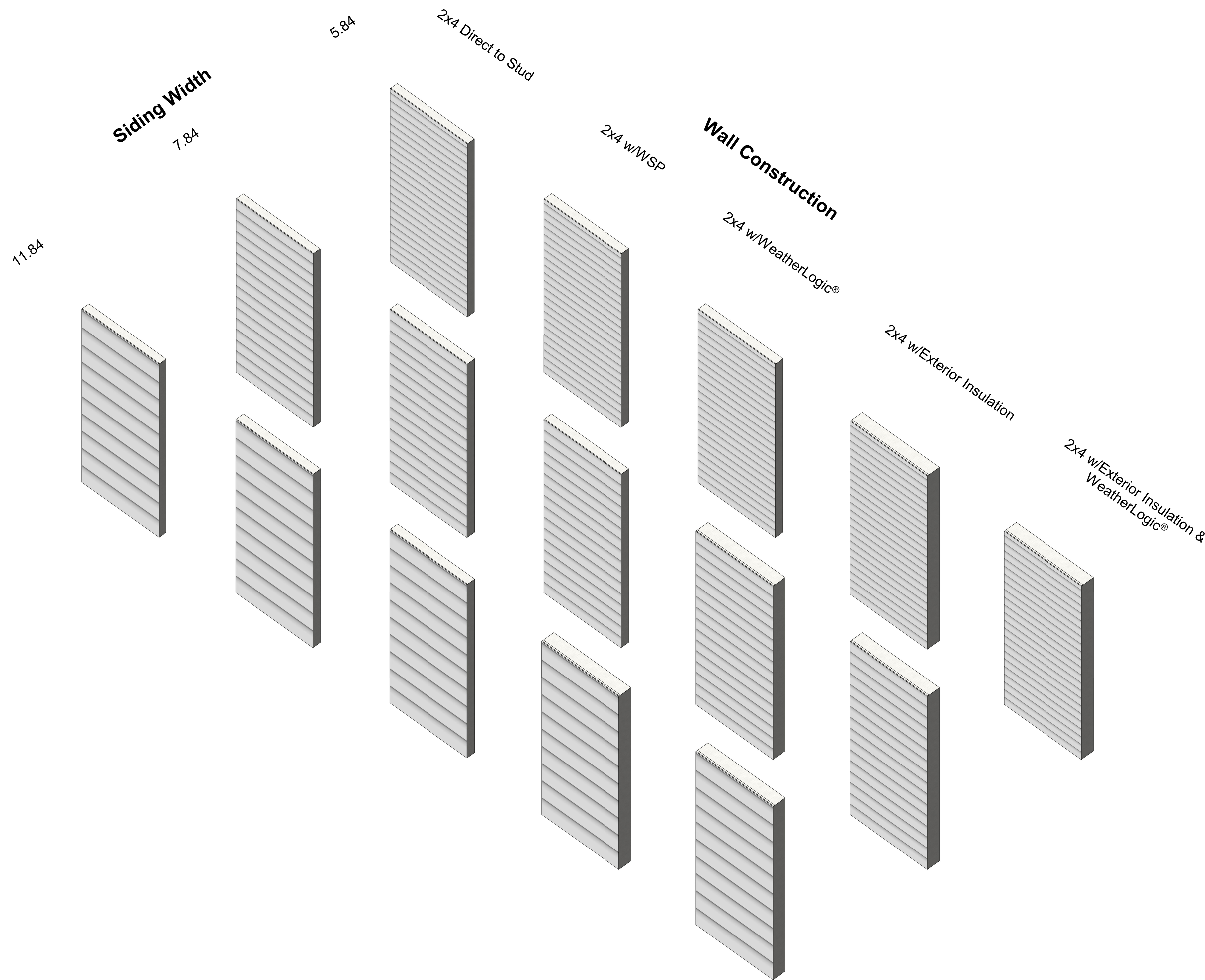
① Wall Types 14 - 76 Series Smooth Finish Lap (Fiber)
