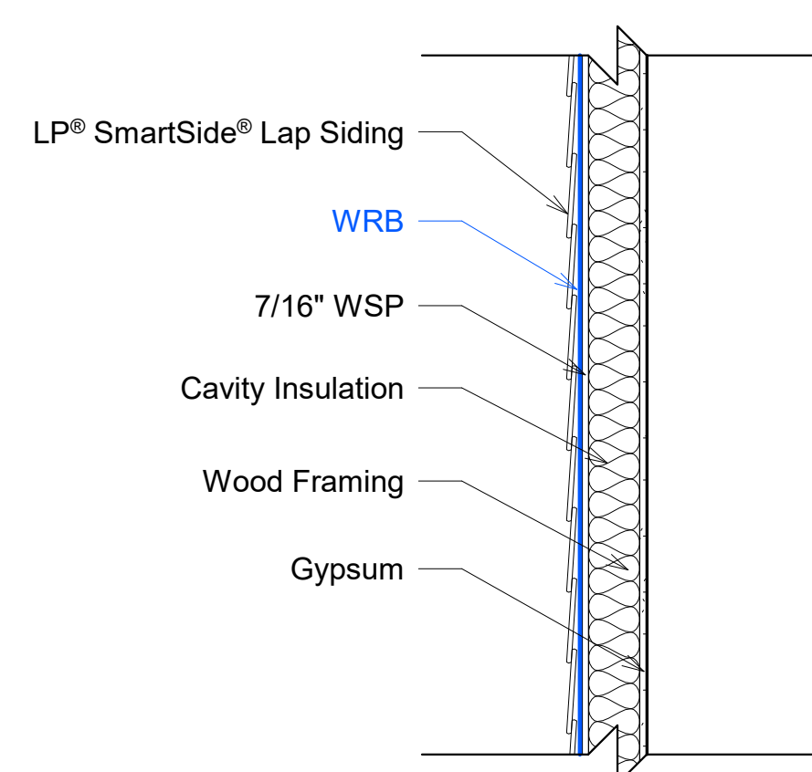
⑤ Section 2 - WSP Application 1" = 1'-0"
