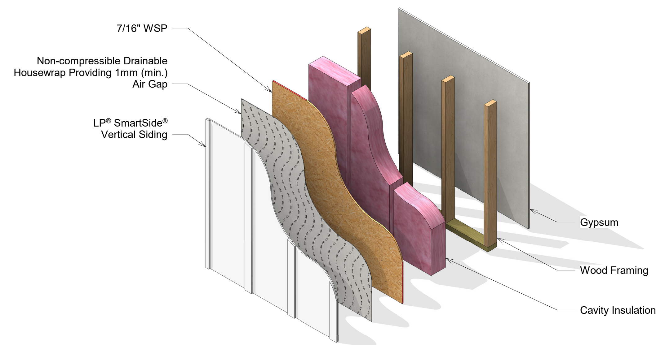
1 Exploded Isometric 1 - WSP Application
