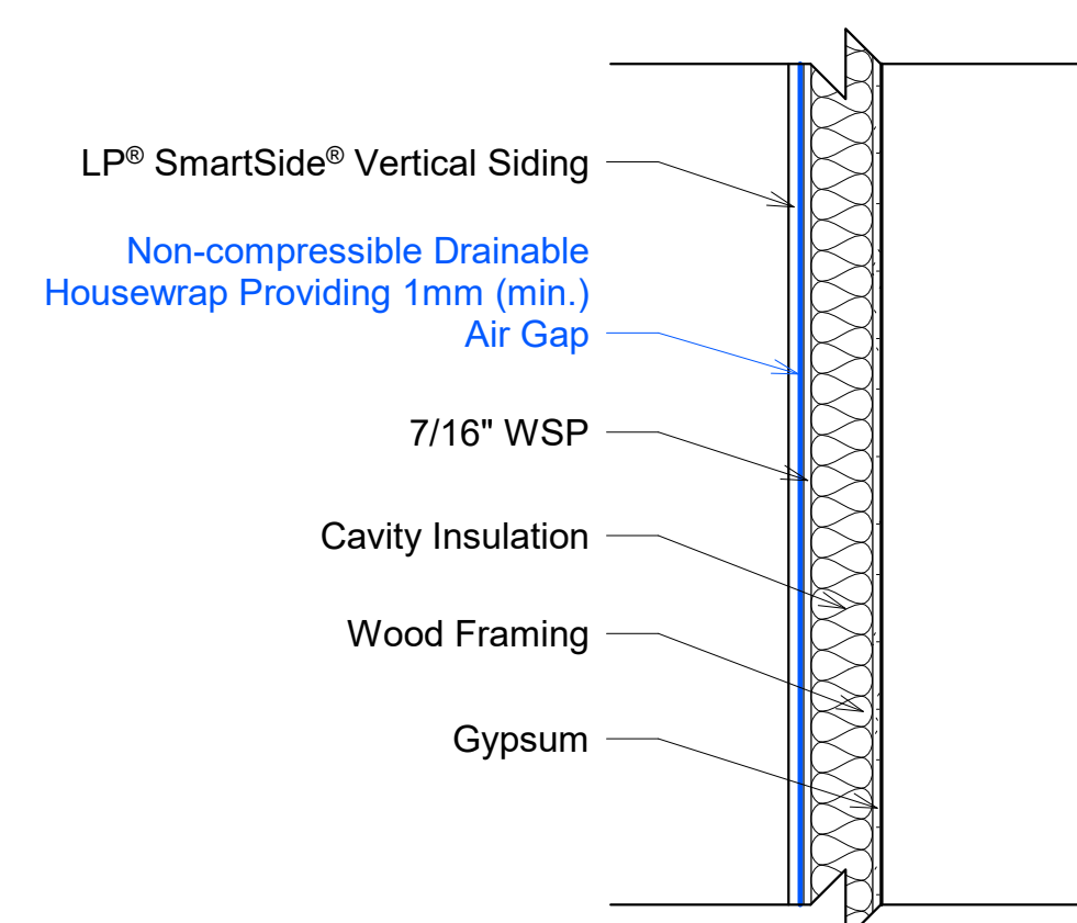
2 Section 1 - WSP Application 1" = 1'-0"
