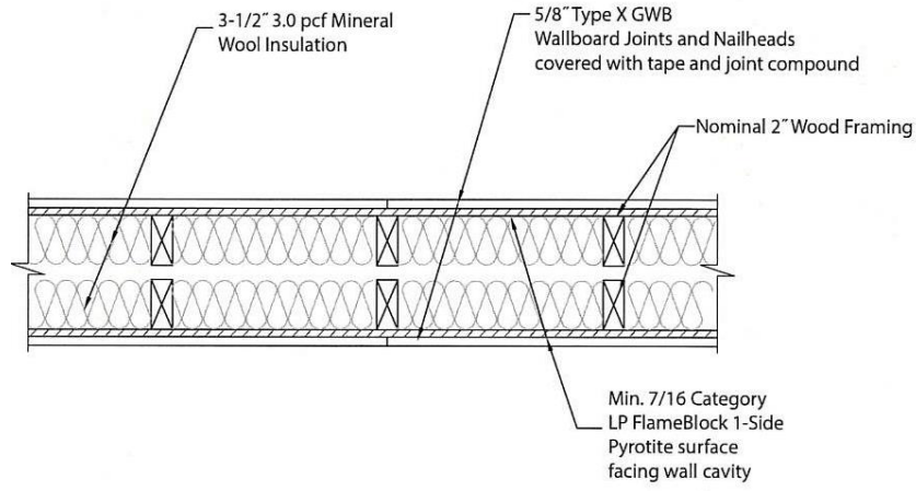
HORIZONTAL SECTION DESIGN No. - UL BXUV.U350 2-HOUR INTERIOR PARTY WALL STC Rating = 61 Configuration A
