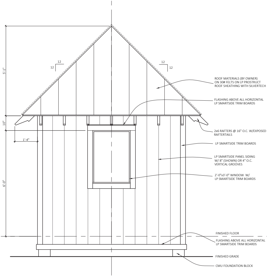
Rear Elevation
