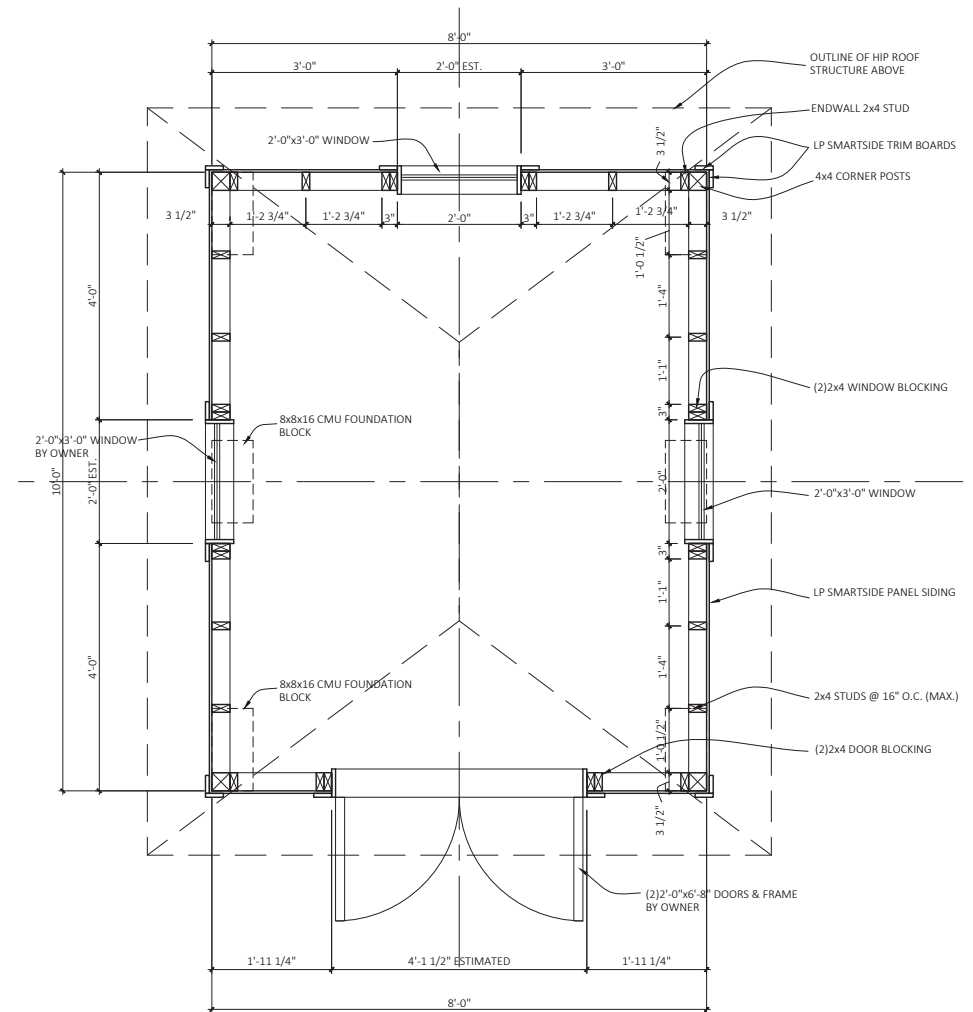
Floor Plan
