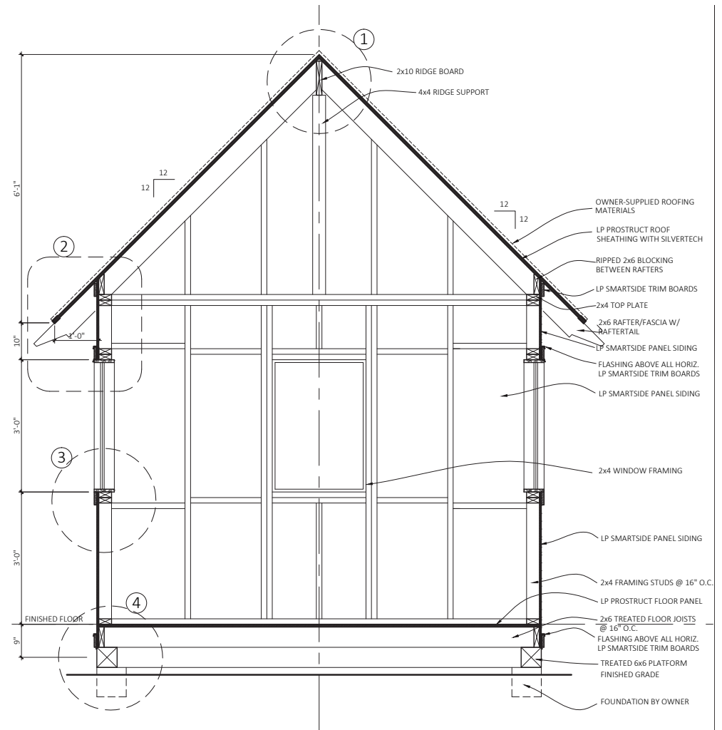
Cross-Section
