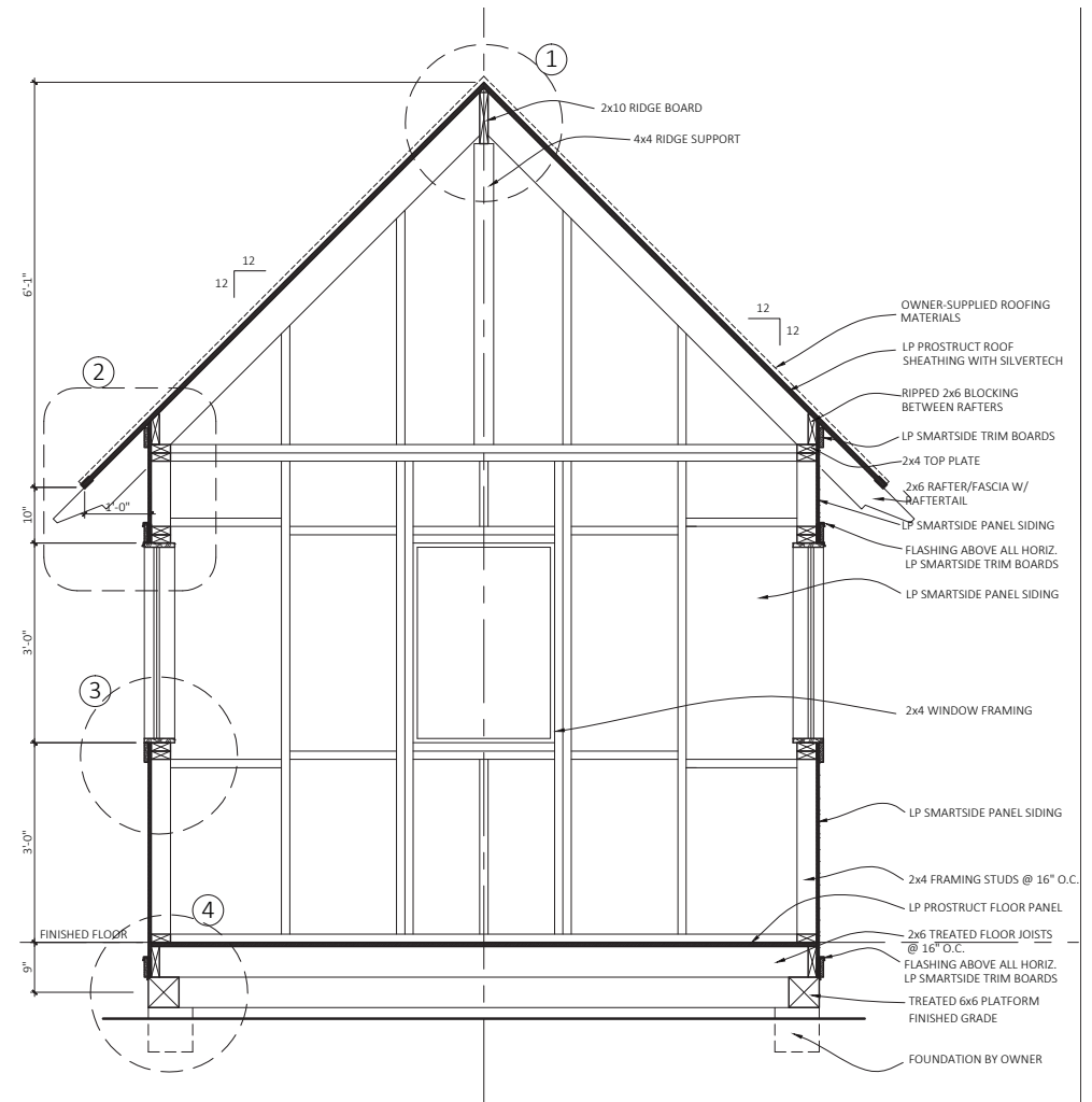
Cross-Section
